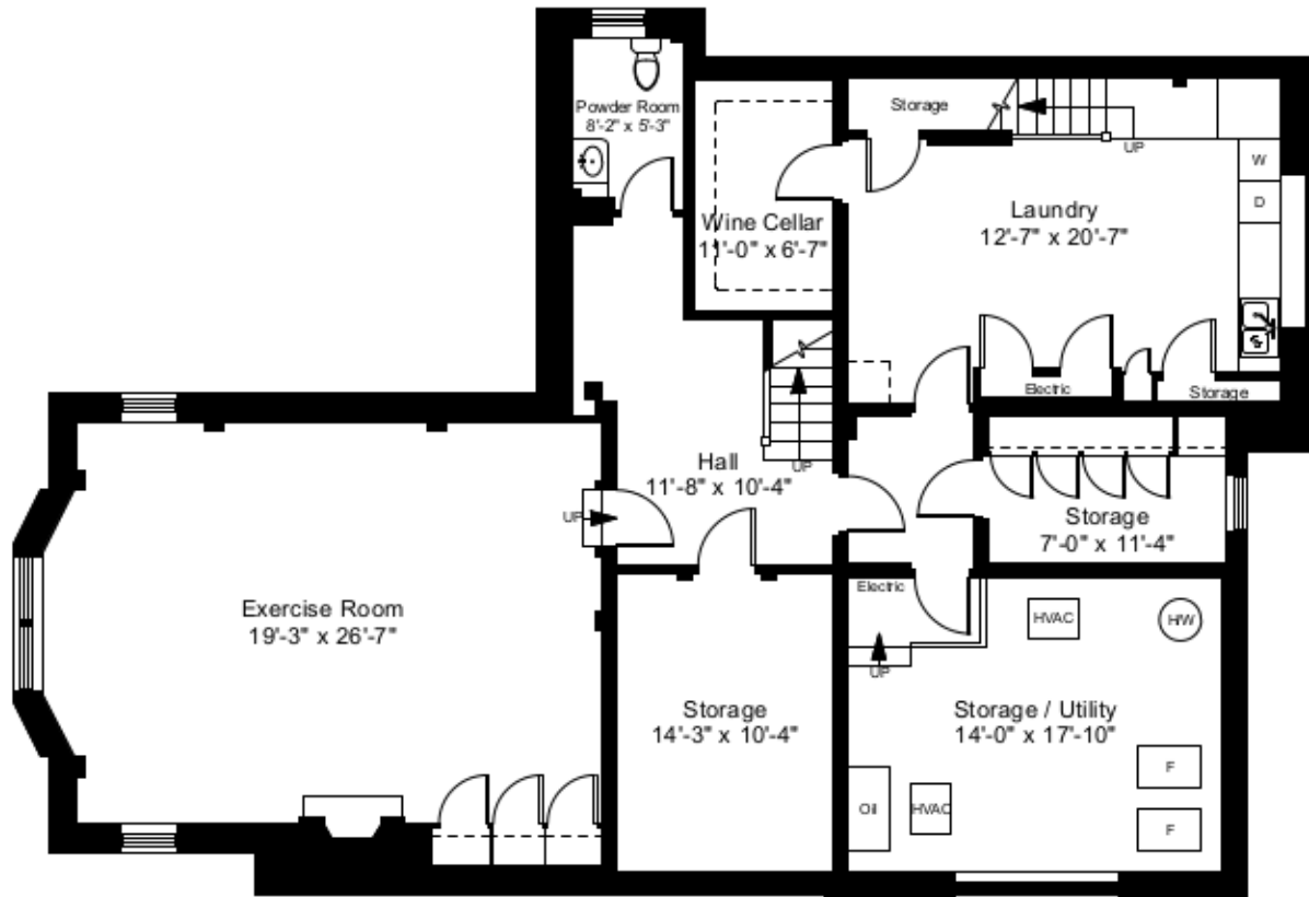
Lower Level Plan Ceiling Height = 7'-2"
