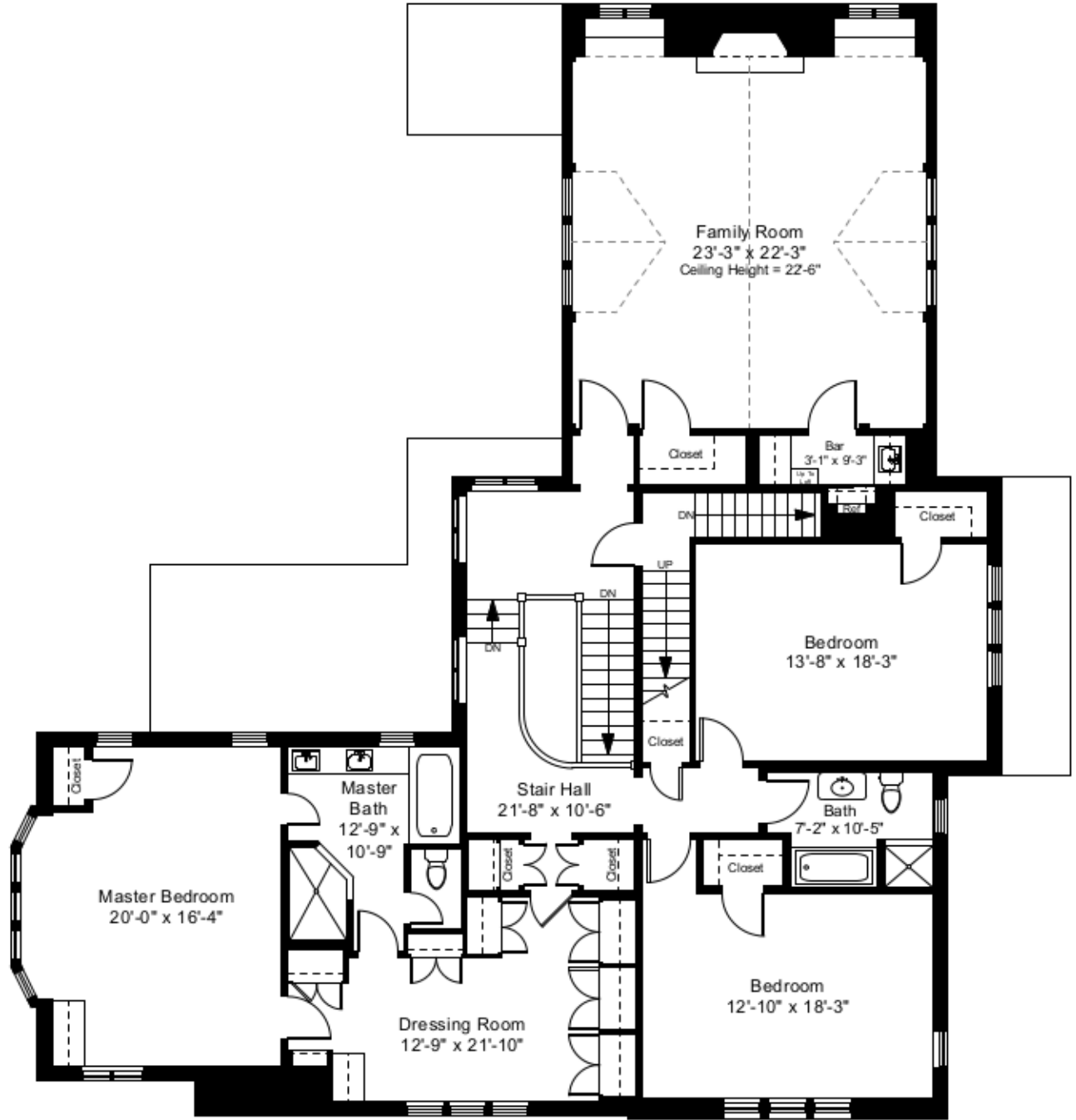
Second Floor Plan Ceiling Height = 8'-0"
